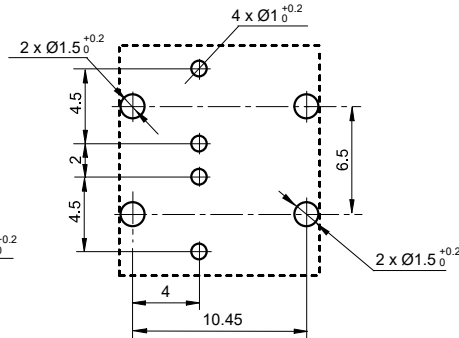
2 Form C (Twin(8 pins)) relay
