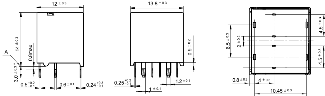
2 Form C (Twin(10 pins)) relay
